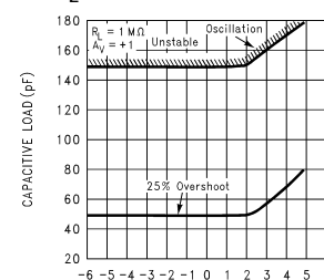
Stability vs Capacitive Load, R_L = 1M\Omega
